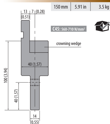
INT100 1000 kN/m max.
