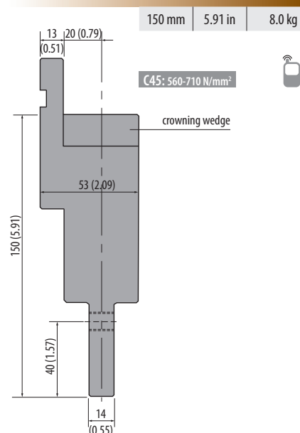
INT150-40 1000 kN/m max.
